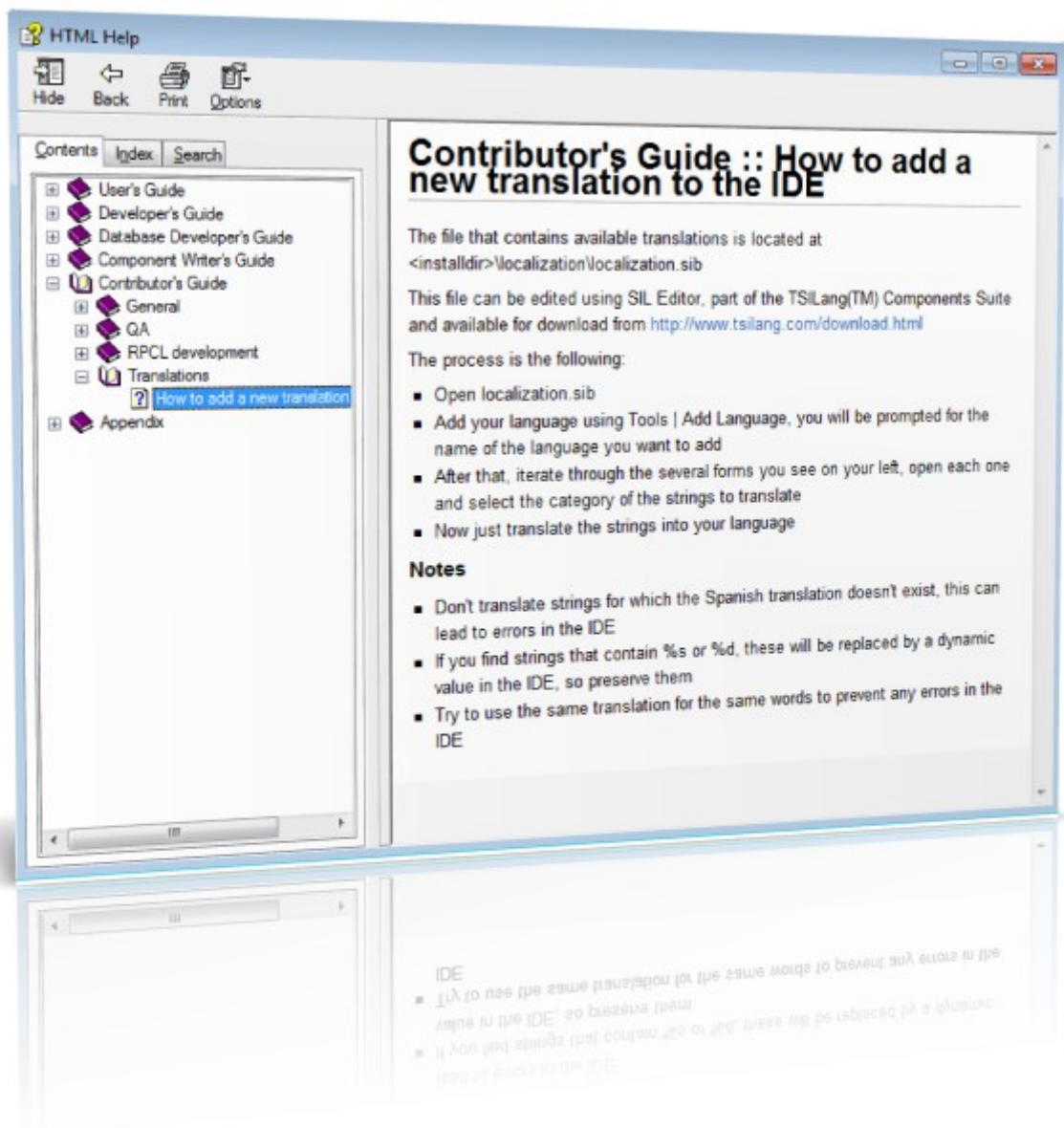
Figure 3. Contributor Guide
