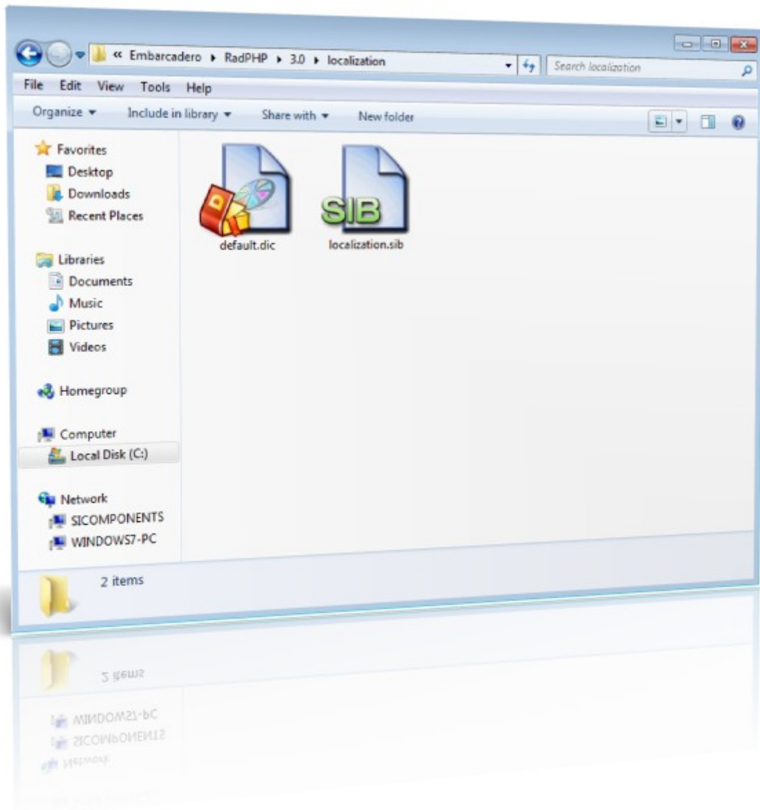
Figure 2. Translation files
