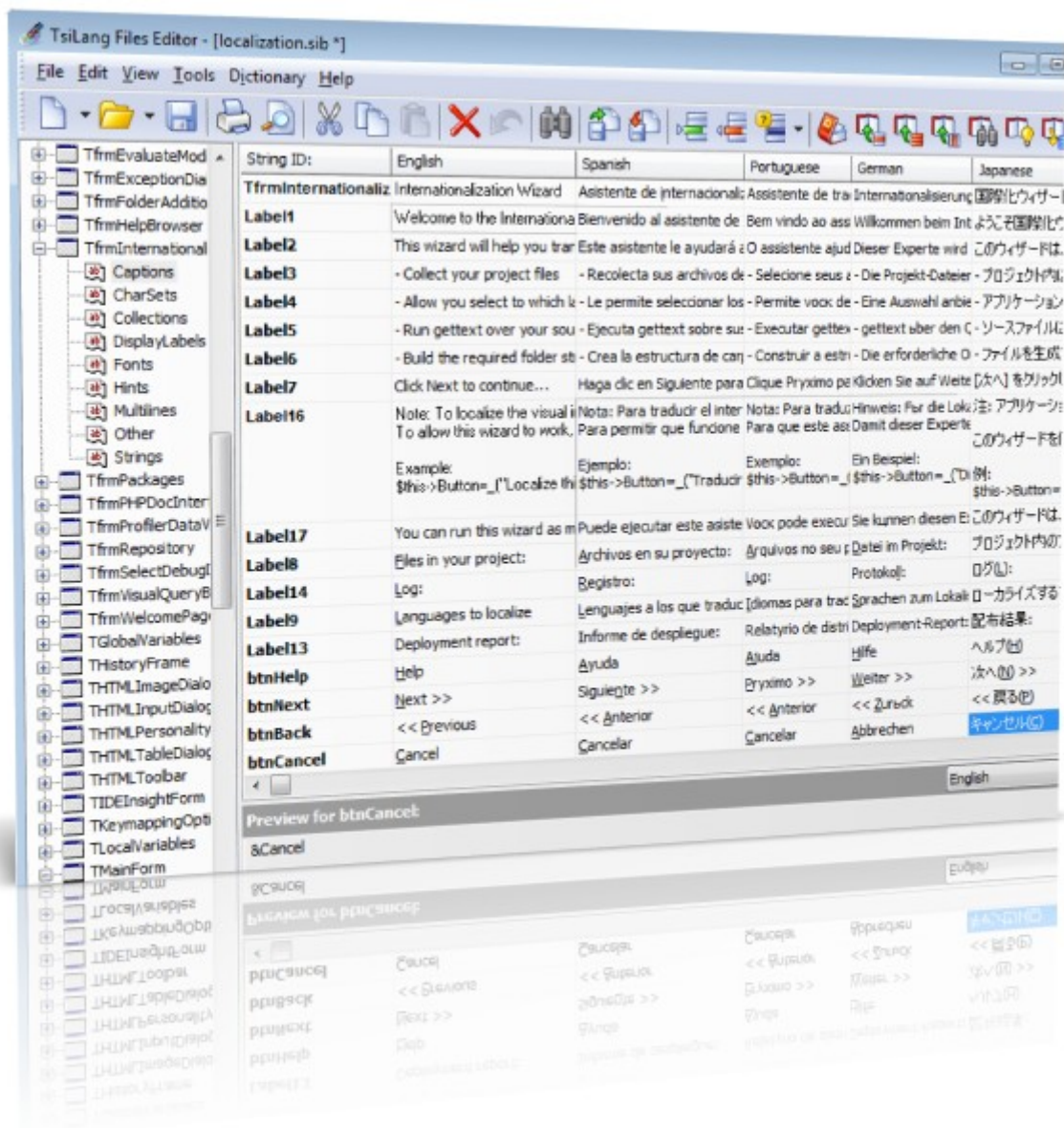
Figure 4. Translation Editor
